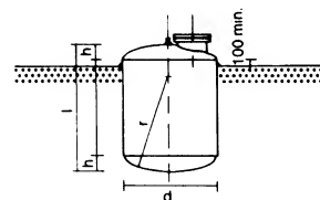
6 Storage tank for heating oil (front view)
